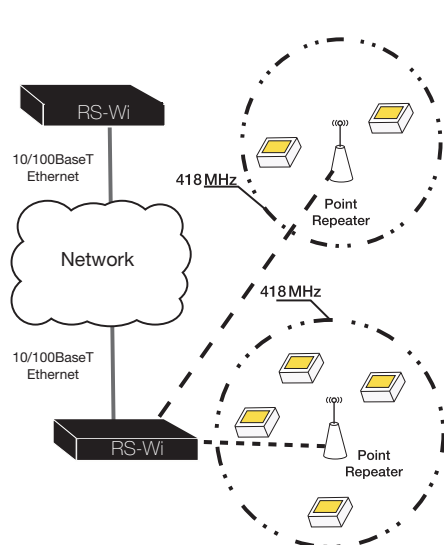
RS-Wi in a Wireless Mesh Network
