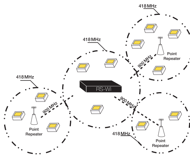
RS-Wi as a Network Repeater
